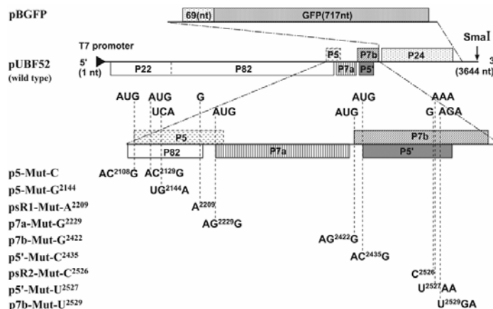
Fig. 1 BBSV cDNAs used for in vitro transcription.
