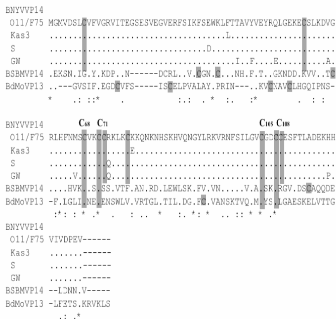
Fig. 2. Amino acid sequence alignment of the cysteine-rich proteins encoded by benyviruses. Cysteine residues were shown in gray background. Asterisks are used to indicate conserved amino acids. The sequence data were collected from DDBJ under the following accession numbers: BNYVV-S D84411, BNYVV-Kas3 AF197556, BNYVV-F75 AF197547, BNYVV-GW X04197 and BSBMV AF061869. The sequences of BNYVV-O11 and BdMV were unpublished.
