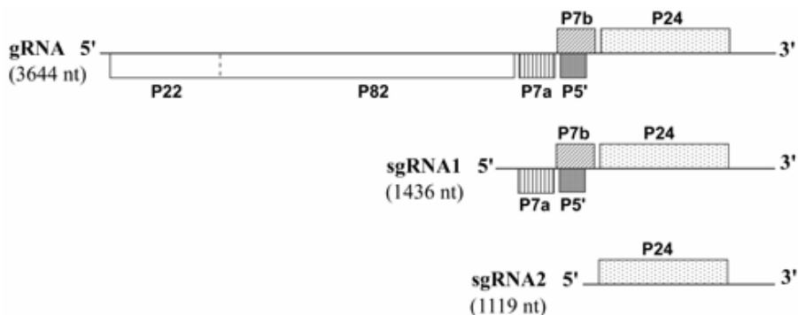
Fig. 5 Proposed BBSV genomic organization and subgenomic expression.
