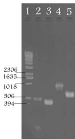
Fig. 1. Detection of BNYVV by RT-PCR. Ethidium bromide-stained agarose gel of RT-PCR products using specific oligonucleotide primers designed to amplify various regions on BNYVV RNA 1 to 4. Lane 1 molecular weight marker, Fermentas (Lithuania), lane 2, RNA 1 (500 bp); lane 3, RNA 2 (430 bp); lane 4, RNA 3 (859 bp); lane 5, RNA 4 (602 bp).
