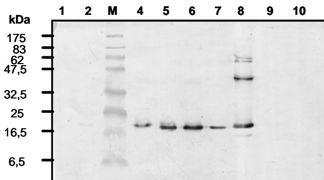
Fig. 1. Western blot analysis of CPs of SBWMV and SBCMV isolates probed with PAS 45 to SBWMV-ATTC type strain. Lanes: 1 healthy rye, 2 SBCMV-Eickeloh, M protein marker, 4 SBWMV type (rye), 5 SBWMV type (wheat), 6 SBWMV-Heddesheim (rye), 7 SBWMV-Heddesheim (wheat), 8 SBWMV-Heddesheim purified virus preparation, 9 healthy wheat, 10 buffer control
