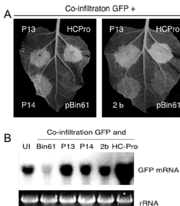
Fig. 1. Suppression of local GFP silencing by benyvirus CRPs. GFP-transgenic N. benthamiana (16c) was agroinfiltrated with the pBin-GFP gene and pBin-P13, pBin-P14, pBin-HCPro, pBin-2b or pBin61. (A) GFP fluorescence visualized under UV-light irradiation. The infiltrated plant was kept at 23°C for 5 days. (B) Northern analysis of GFP mRNA in infiltrated zones. UI: uninfiltrated 16c leaves. The lower panel shows ethidium bromide (EtBr) staining of the same samples.
