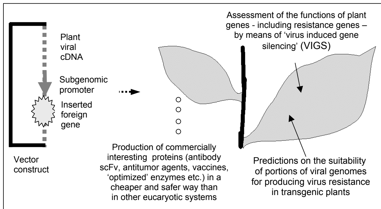
Fig. 1. Various applications of plant viral vector constructs
