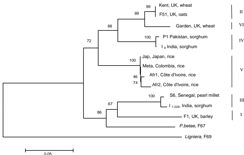
Figure 1. Phylogenetic tree of the ITS5-ITS4 rDNA regions obtained using Neighbour Joining analysis (Tamura-Nei distances) in the package MEGA3 (Kumar et al. , 2004). Percentage bootstrap values (1000 replicates) are shown above the forks.
