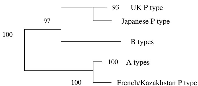
Fig. 3 A simplified cluster tree for RNA4 sequences showing groupings of P, A and B types of BNYVV. The tree was rooted with Beet soil-borne virus (not shown). The values indicate the number of times out of 1000 that this grouping occurred after bootstrapping the data.
