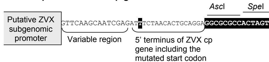
Fig. 3. Various alternatives used to introduce the Ascl and Spel sites needed for the insertion of foreign genes into the ZVX-based vector sequence downstream of the putative ZVX coat protein (cp) subgenomic promoter and ability of the resulting constructs pA, pB and pC to express inserted BNYVV cp gene in infected plants. The Ascl and Spel sites and the 'T' replacing the original 'G' in the ZVX cp start codon in pC are highlighted by white letters on a black background. Bar represents 100 nm. Magnification are the same in both electronmicrographs.
