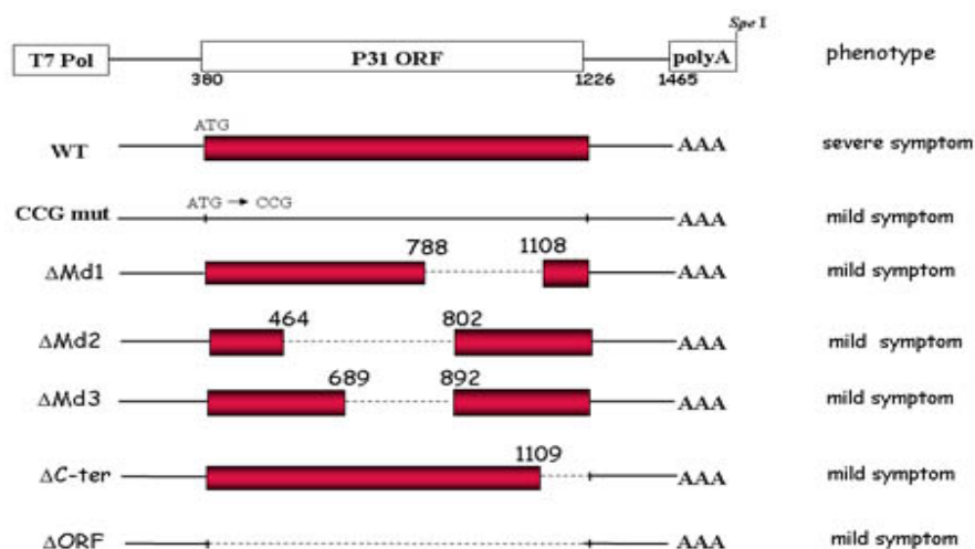
Figure 1. Genetic map of BNYVV RNA 4 mutants and symptom phenotypes in N. benthamiana .
