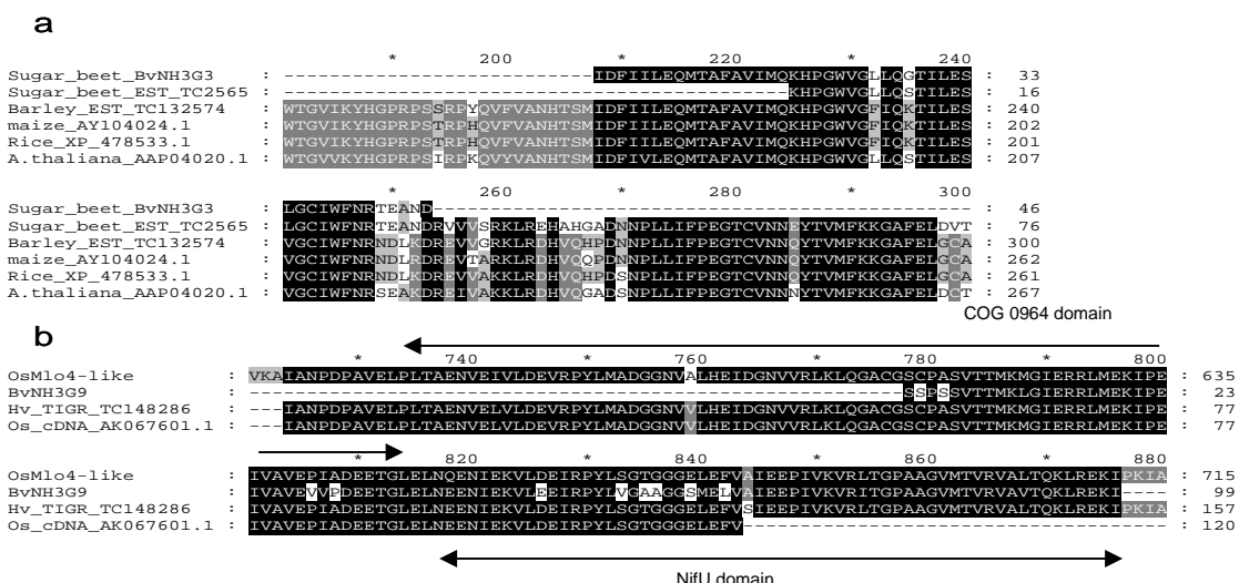
Fig. 2 Protein sequences alignments for BvNH3G3 (a) and BvNH3G9 (b). Identical amino acids are shaded in black, similar amino acids in grey.
