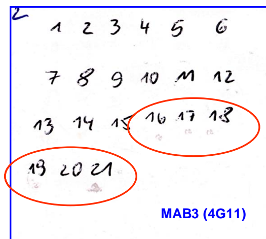
Fig. 2. Comparison of TPIA and ELISA systems for detection of SBCMV in 21 samples: 1-7 positive for Wheat spindle streak mosaic virus in DAS-ELISA, 7-12 healthy plants, 13-15 positive for SBWMV in DAS-ELISA based on MAB 4G4, 16-21 positive for SBCMV in TAS-ELISA using MAB 4G11.
